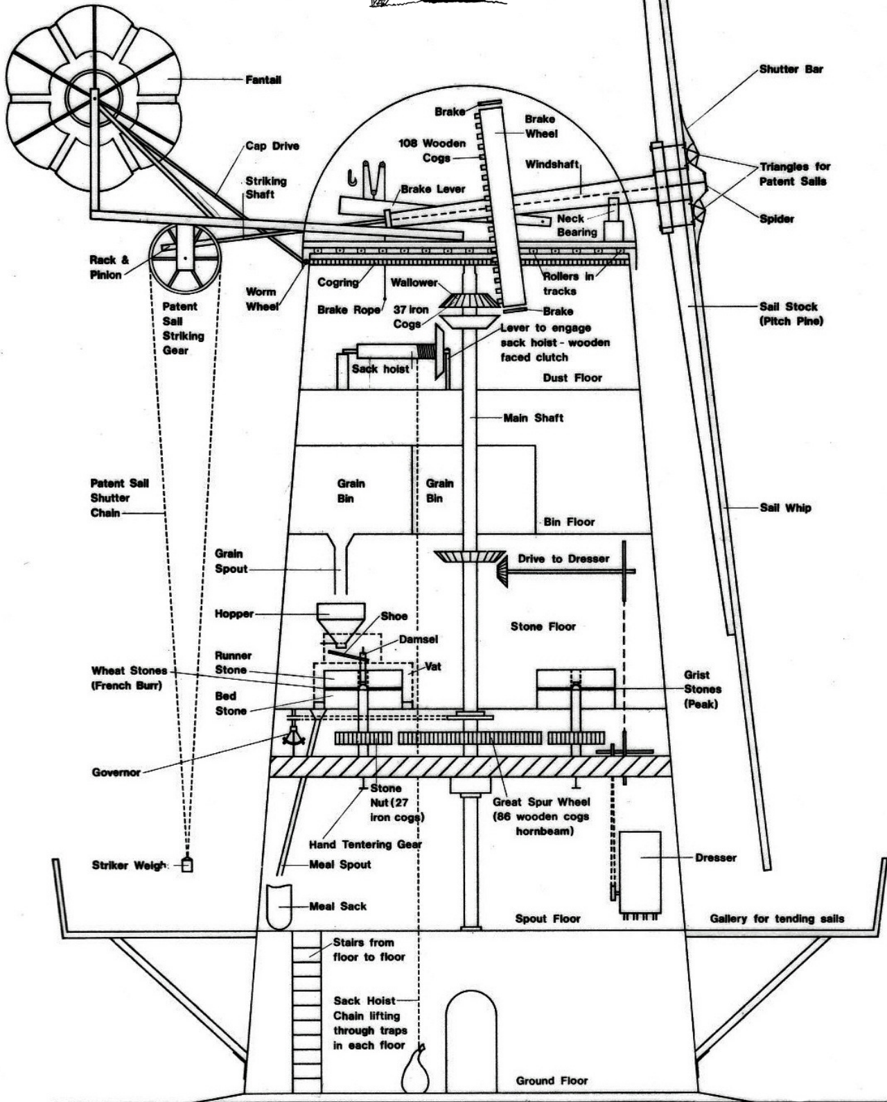
A CROSS SECTION THROUGH WILTON WINDMILL
